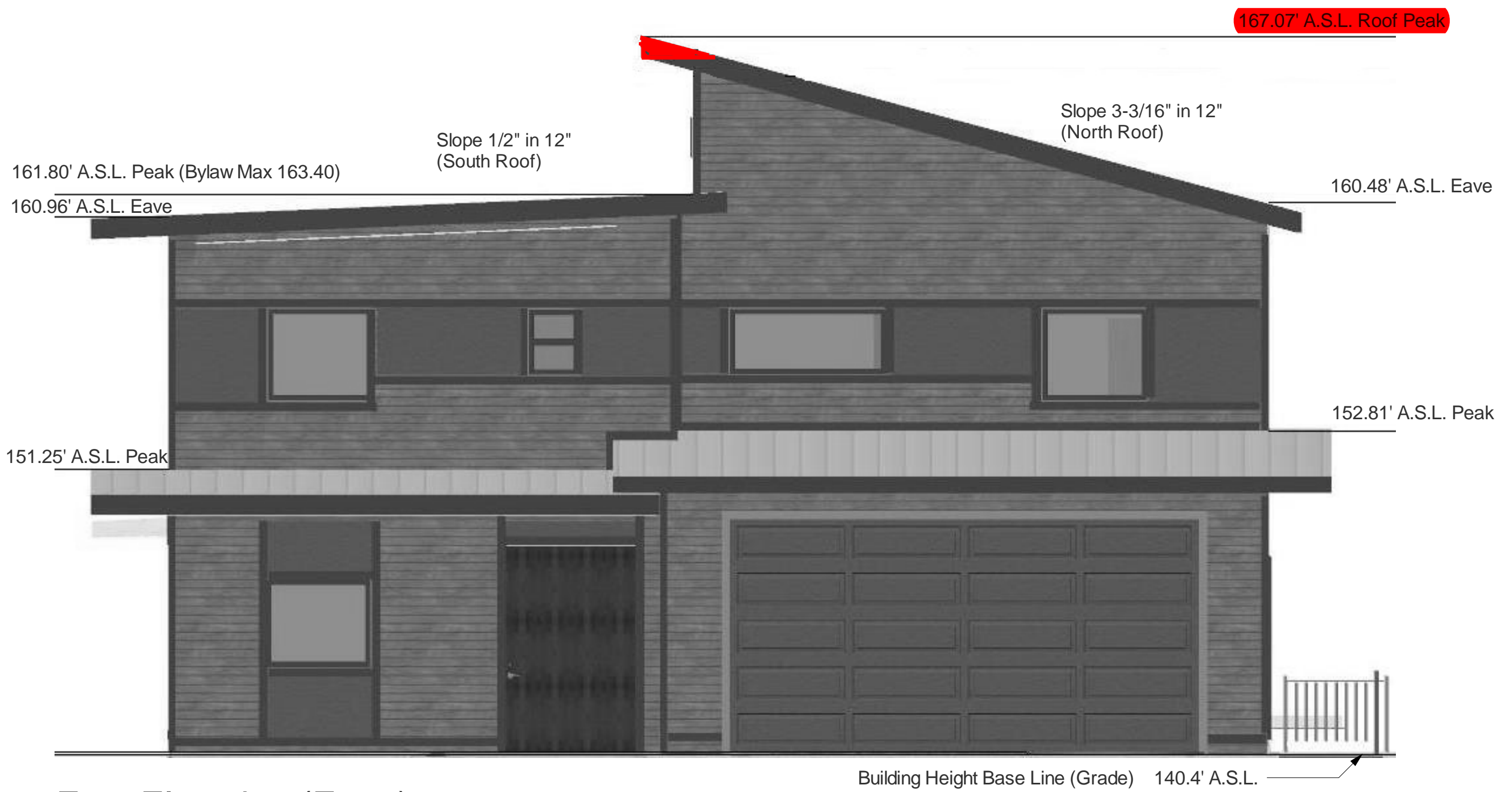
East Elevation (Front)
